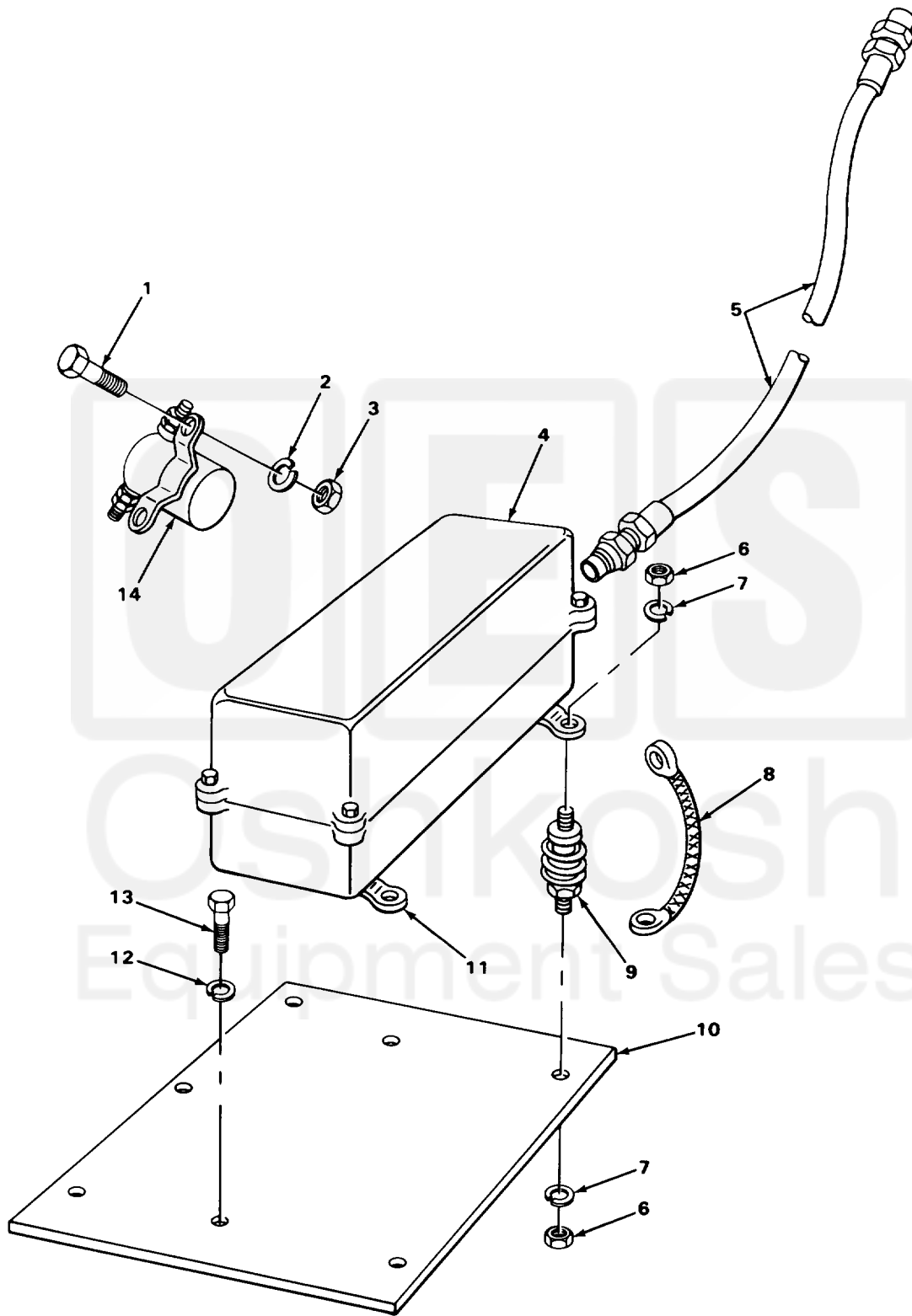
FIGURE 31. VOLTAGE REGULATOR.
